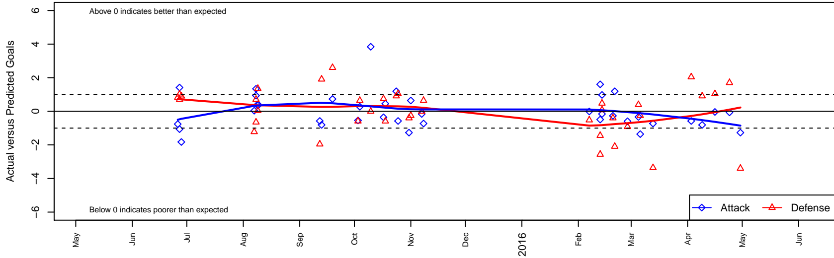
Bend FC Timbers Red B01 Dots are actual minus expected GF (blue circles) and GA (red triangles). Blue line is smoothed change in attack strength. Red is smoothed change in defense strength.
